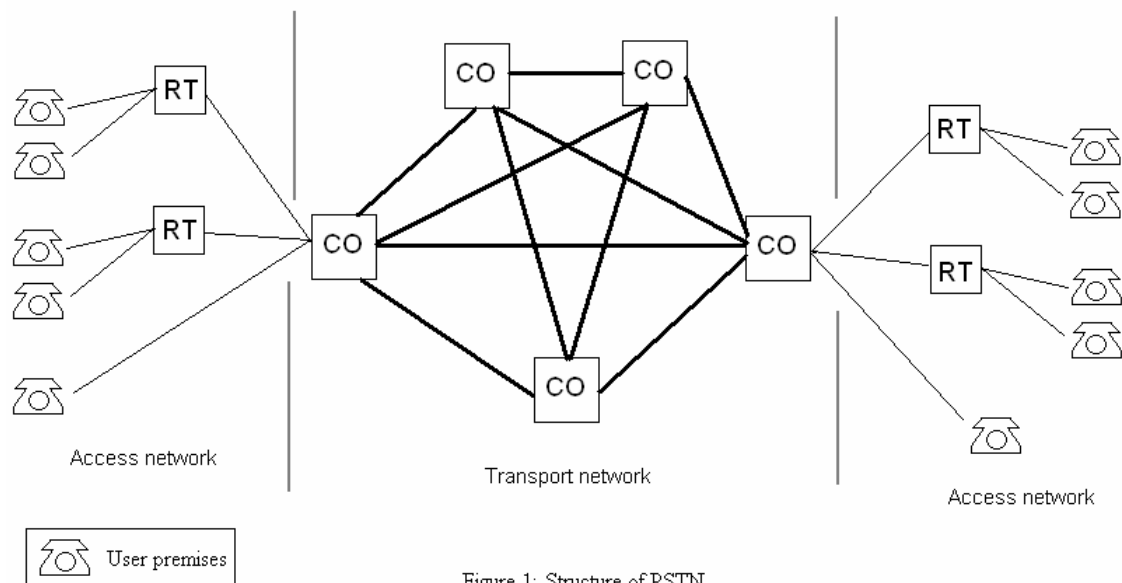
Figure 1: Structure of PSTN
